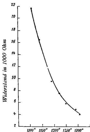
Fig. 6. Quarz III.
